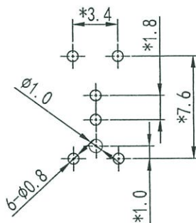
PCB Layout Component Side Shown
